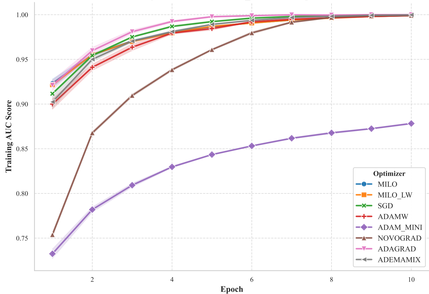
Training AUC for RESNET34_CIFAR10 Experiment
